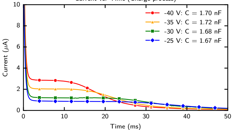
Current vs. Time (Charge process)
